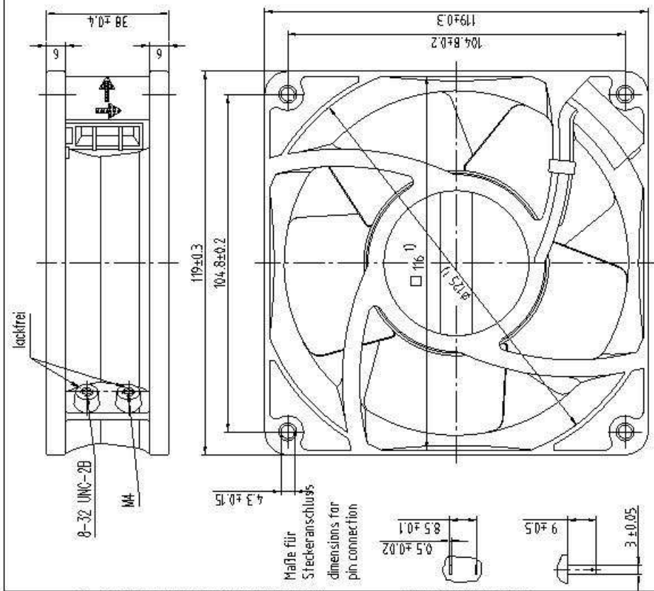
1) dimensions for assembly wall
