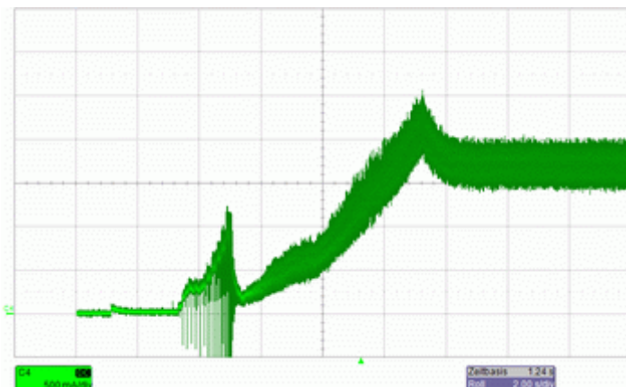
Start-up current @ 24 V (I = 500mA/div ; t = 2s/div)
