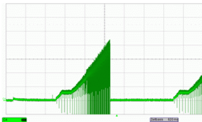
Locked rotor current @ 24 V ( I = 0,5\text{A/div} ; t = 1\text{s/div} )
