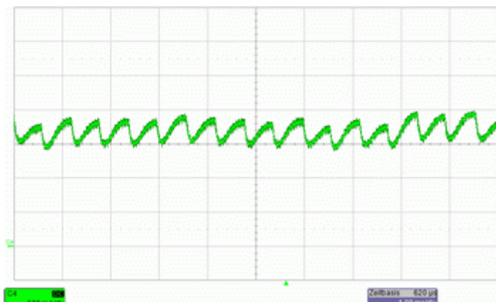
Running current @ 24 V ( I = 500\text{mA/div} ; t = 1\text{ms/div} )
