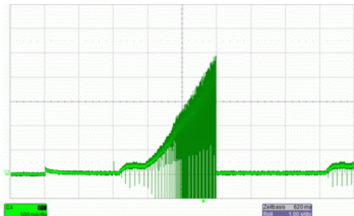
Locked rotor current @ 36 V ( I = 0,5\text{A/div} ; t = 1\text{s/div} )
