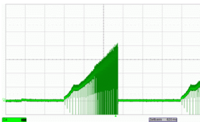
Locked rotor current @ 16 V ( I = 0,5\text{A/div} ; t = 1\text{s/div} )
