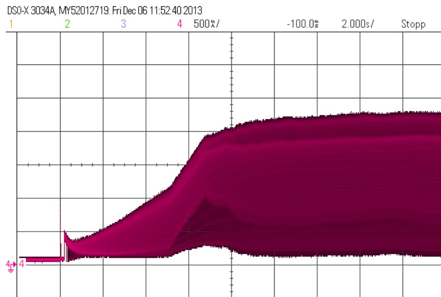
Running current @ 24 V ( I = 500\text{mA/div} ; t = 2\text{ms/div} )
